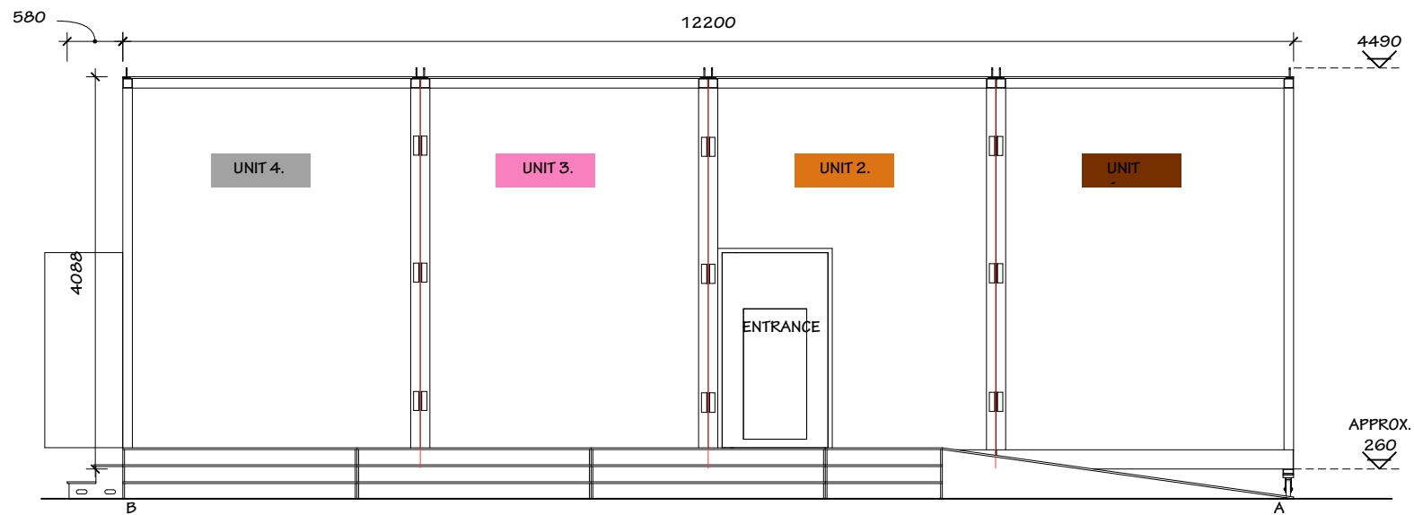
MAGIC LIBRARY. ELEVATION B-A. SCALE 1 : 50.
