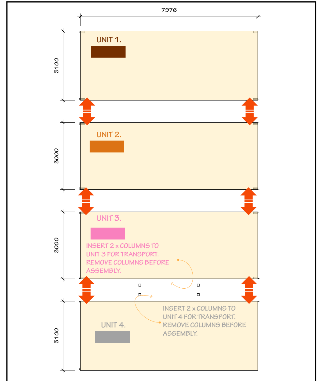
EXTERIOR TOP VIEW OF UNITS SEPARATED.
