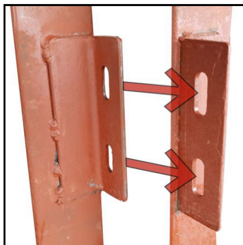
CONNECTOR TABS.
