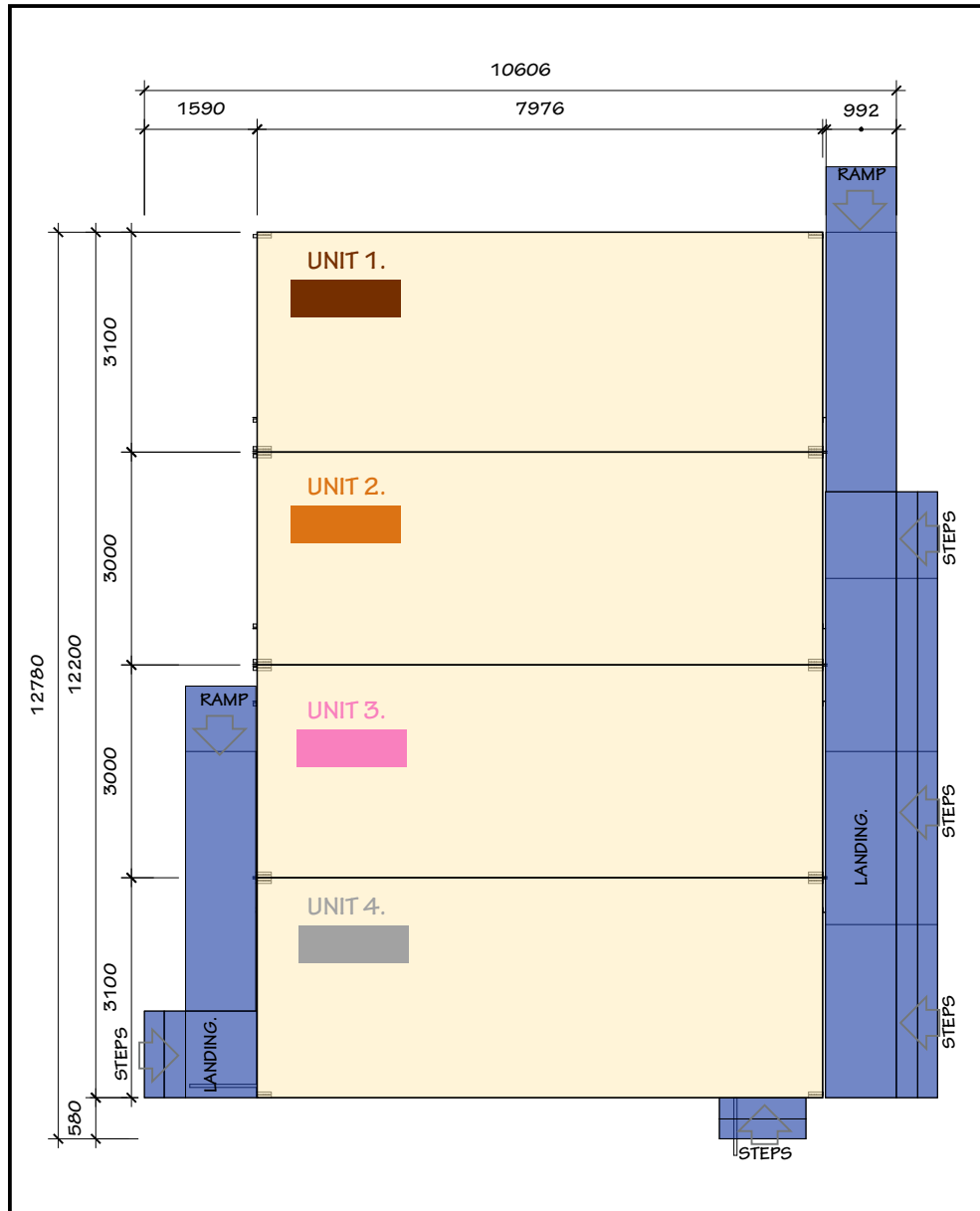
EXTERIOR TOP VIEW OF UNITS ASSEMBLED.
